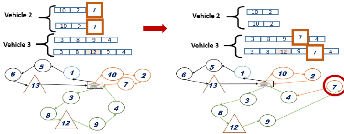
Figure 3. Insert Moves
