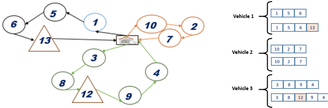
Figure 2. Solution Representation
