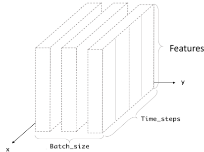
Figure 4. GRU input shape
