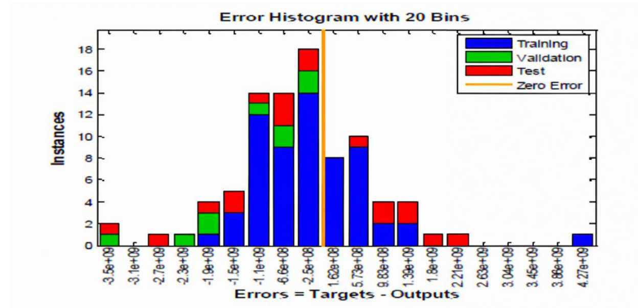
Figure 6. LMBP neural network error histogram
