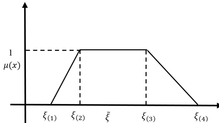
Figure 2. The trapezoidal possibility distribution of fuzzy parameter \tilde{\xi}
