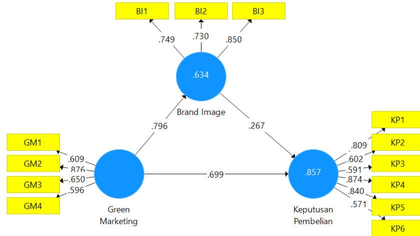
Figure 6. Model Estimation
