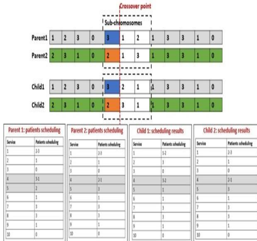
Figure 8: Example of the proposed three steps crossover
