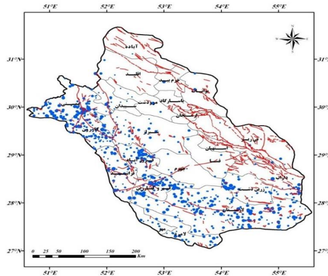
Figure 2. The map of distribution of earthquake centers relative to fault lines
