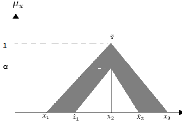
Figure 2. Triangular interval-value fuzzy numbers (Ashtiani et al. 2009)
