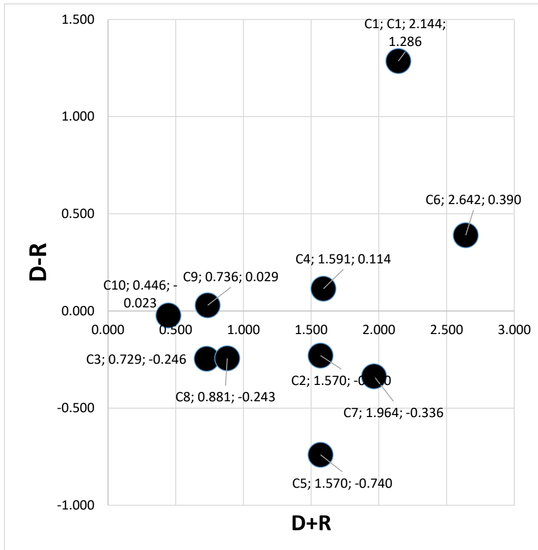
Figure 3. The digraph of causal relations
