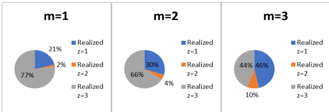
Figure 7. Distribution of utilization times of machines in sub-periods (realized)
