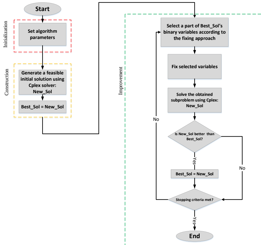
Figure 1. General flowchart of the proposed fix-and-optimize matheuristics
