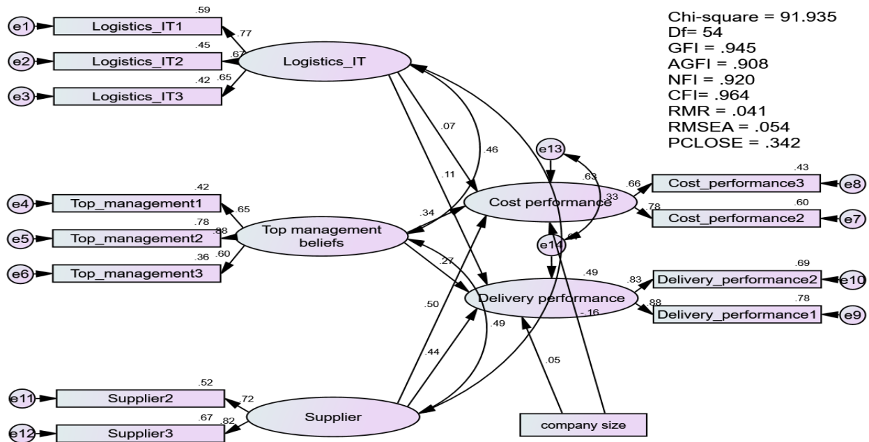
Figure 3. Structural model with parameter estimates.
