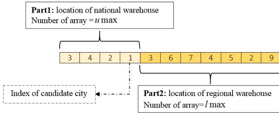
Figure 4. Solution representation
