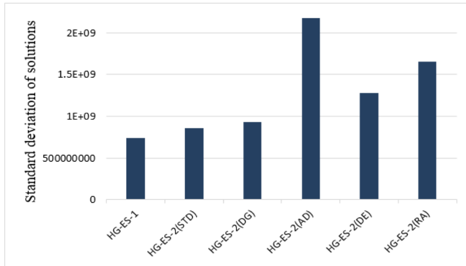
Figure 16. Result of the large-size instance (SDOFU)
