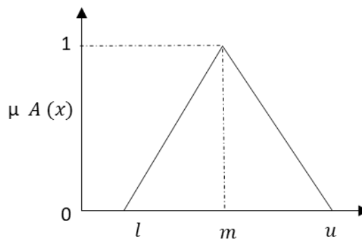
Figure 5. Graphical representation of a triangular fuzzy number
