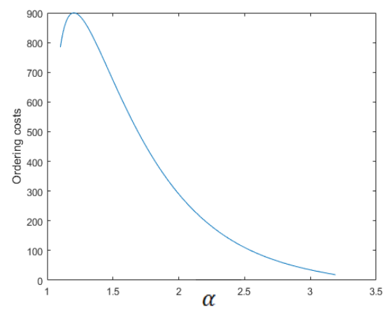
Figure 5. The changes of \alpha versus annual ordering costs
