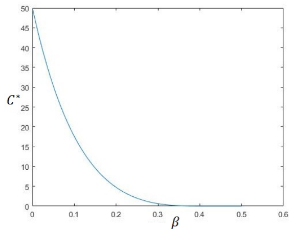
Figure 6. The changes of \beta versus optimal item cost ( C^* )
