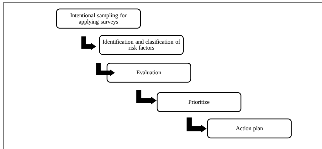
Figure 3. Methodology
