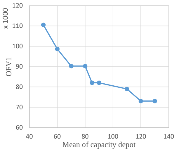
Figure 17. OFV1 vs. mean of capacity depot
