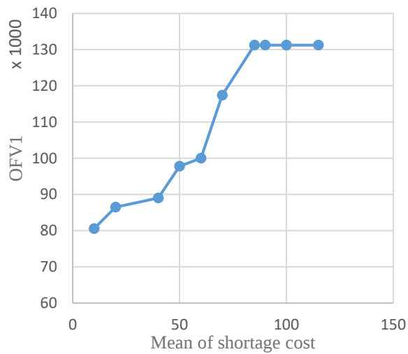
Figure 13. OFV1 vs. mean of shortage cost
