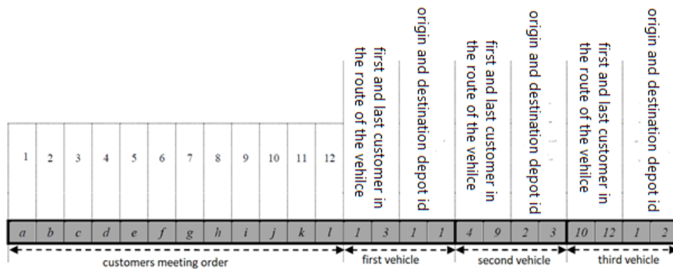
Figure 3. Encoding of the vehicle's routes for each period (Eydi and Abdorahimi, 2012).
