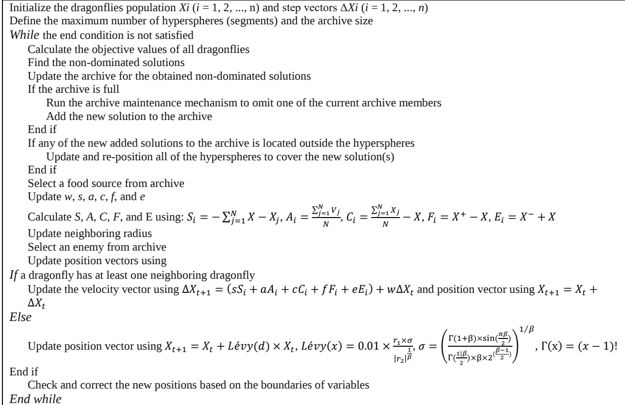
Figure 4. Pseudo-codes of the MODA
