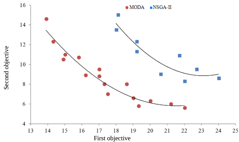
Figure 6. Pareto fronts of two meta-heuristics
