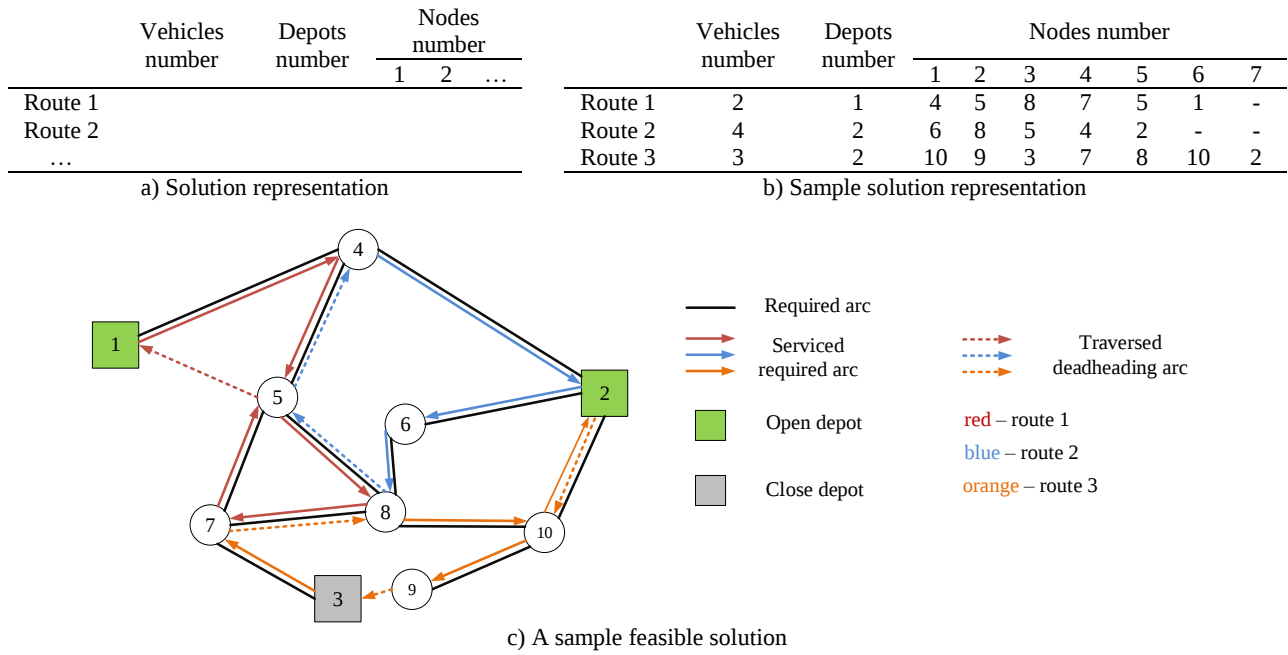
Figure 3. Solution representation with a sample for the proposed LARP
