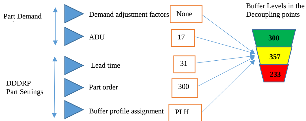
Figure 8. Buffer Level in the Decoupling Point
