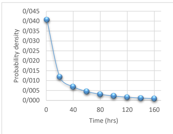
Figure 11. Weibull Pdf for P 201-C
