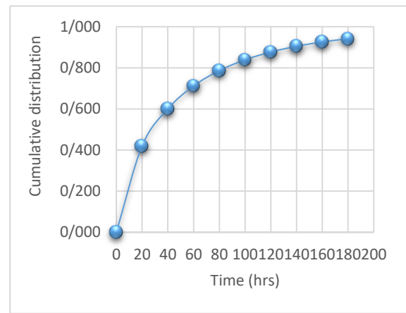
Figure 12. Weibull Cdf for P 201-C
