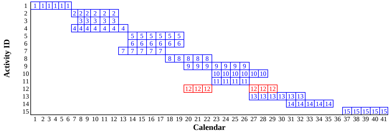
Figure 7. The Gantt of the first experiment after using the heuristic in the condition of confronting with resource limitations
