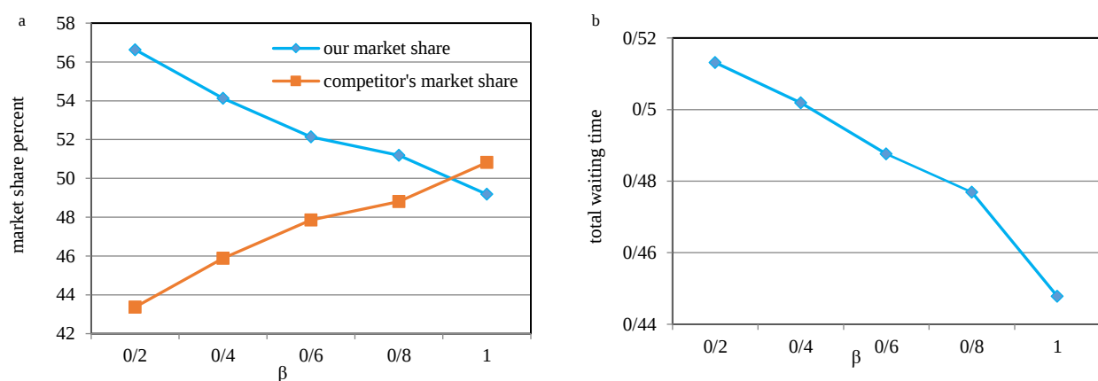
Figure 5. Sensitivity analysis with respect to \beta
