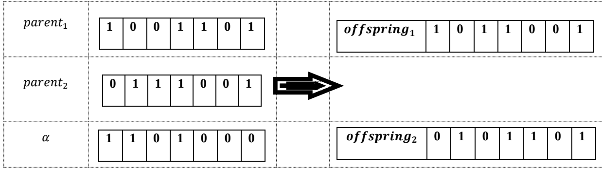
Figure 3. Crossover operator
