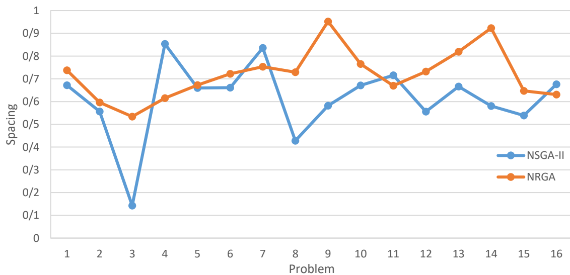
Figure 10. Detailed comparison of spacing metrics on different 16 test problems of NSGA-II and NRGa in Table 20
