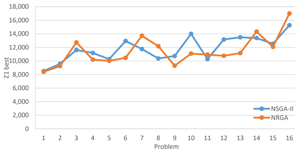
Figure 7. Comparisons between the first objectives function values of NSGA-II and NRGGA in Table 20
