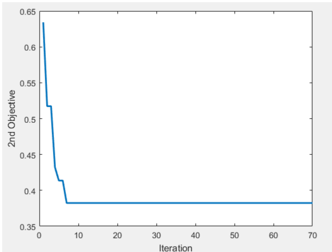
Figure 14. The convergence of NRGa on second objective function
