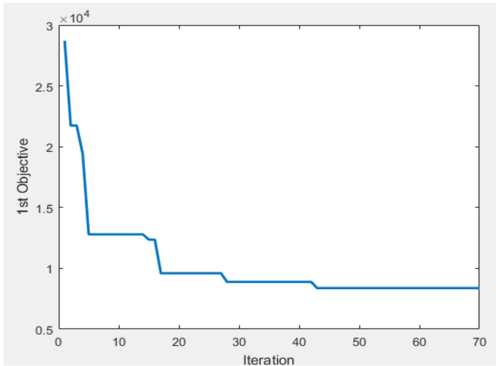
Figure 13. The convergence of NRGa on first objective function
