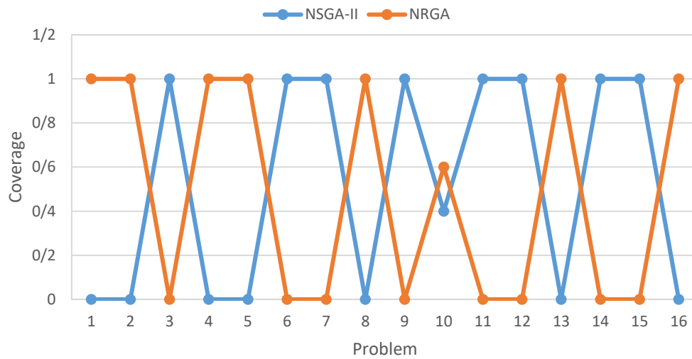
Figure 9. Detailed comparison of coverage metrics on different 16 test problems of NSGA-II and NRGa in Table 20
