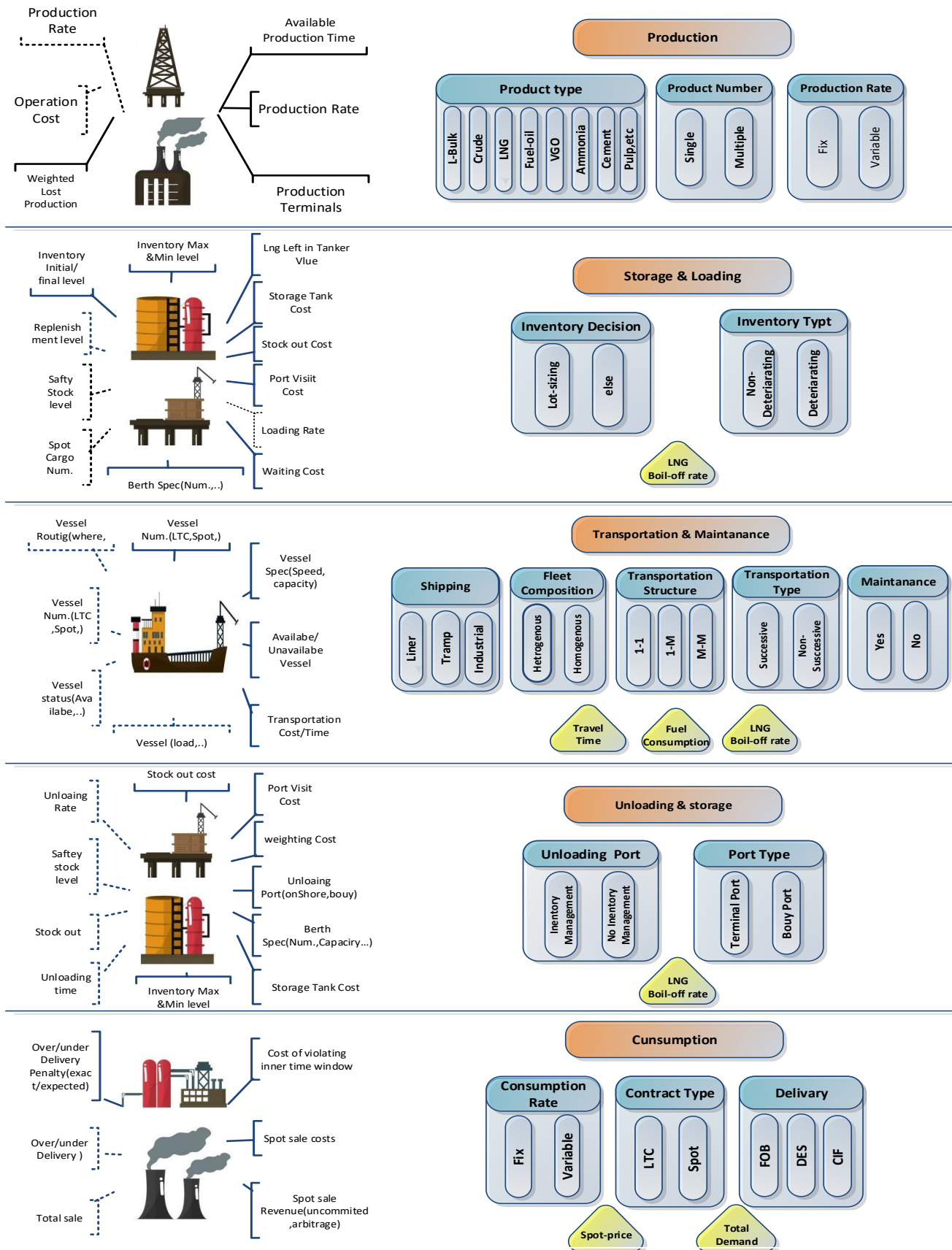
Figure 8. The Conceptual Model of the maritime inventory routing problem
