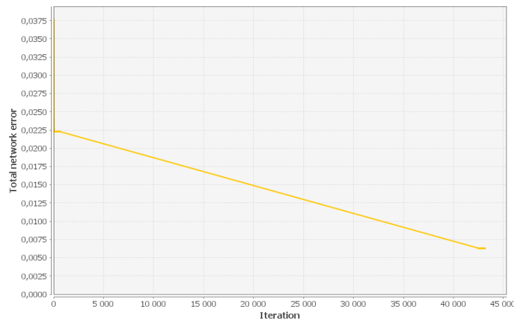
Figure 4. MSE training graph of RBF
