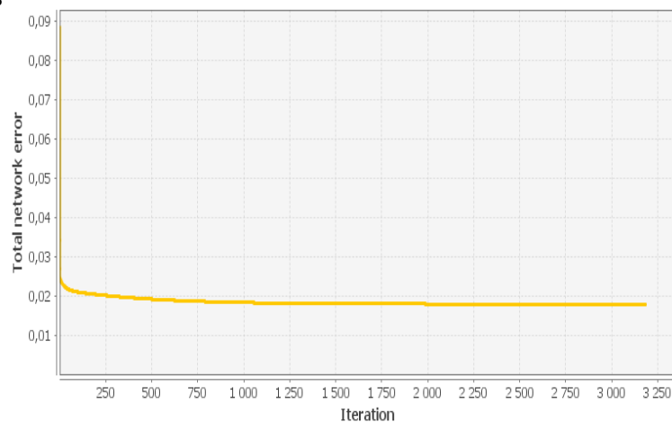
Figure 3. MSE training graph of NoProp
