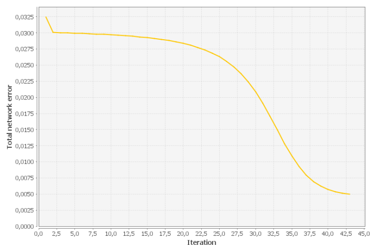
Figure 6. MSE training graph of MLP
