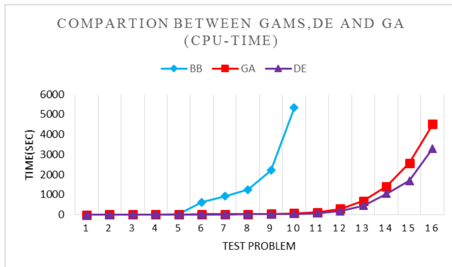
Figure 7. Comparison between CPU times related to the B&B, GA and DE: small and medium-sized problems and large-sized problems
