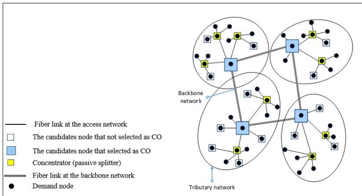
Figure 2. An example of three-layered ring backbone and star/star access network with 4 sector Predetermined
