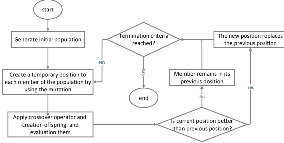
Figure 4. Flowchart of the DE
