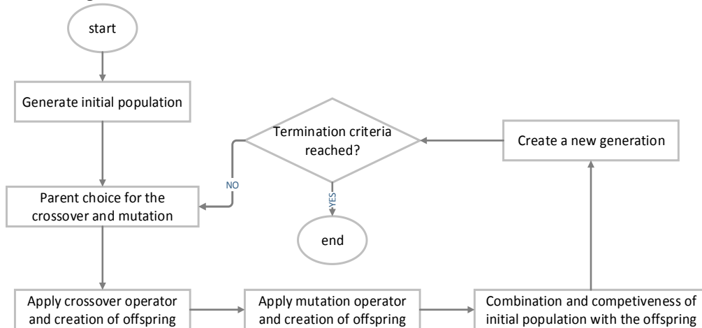
Figure 3. Flowchart of the GA
