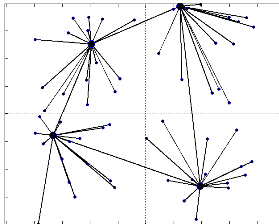
Figure9. Illustration of the example with \alpha = 5
