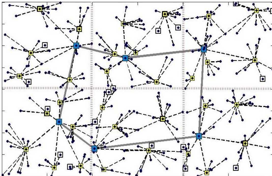
Figure 8. The result of test problem 13 obtained by DE
