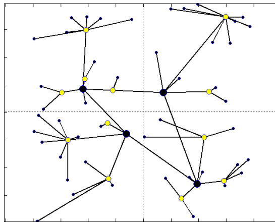
Figure 11. Illustration of the example with \alpha = 0.05
