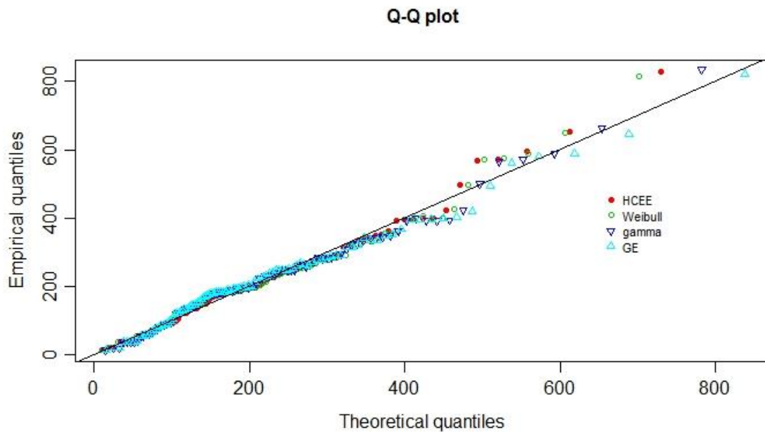
Figure 8(d). Q-Q plots of fitted PDFs for the yarn data set.
