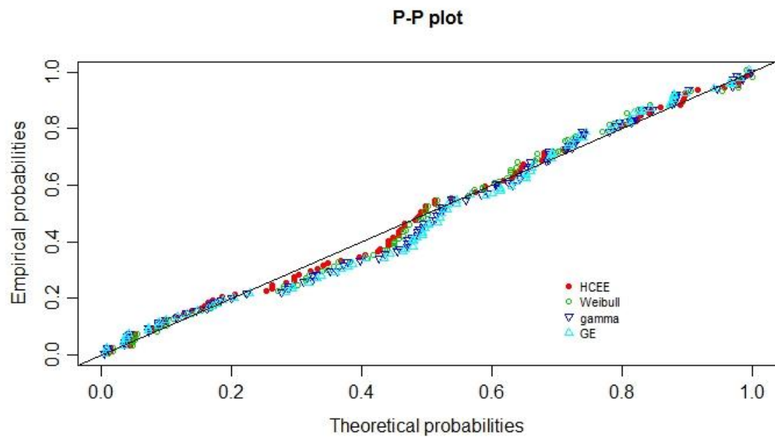
Figure 8(c). P-P plots of fitted PDFs for the yarn data set.
