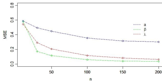
Figure 6. Absolute MSE's of selected parameters( a = 2, \beta = 2, \lambda = 2 ) for HCEE model.
