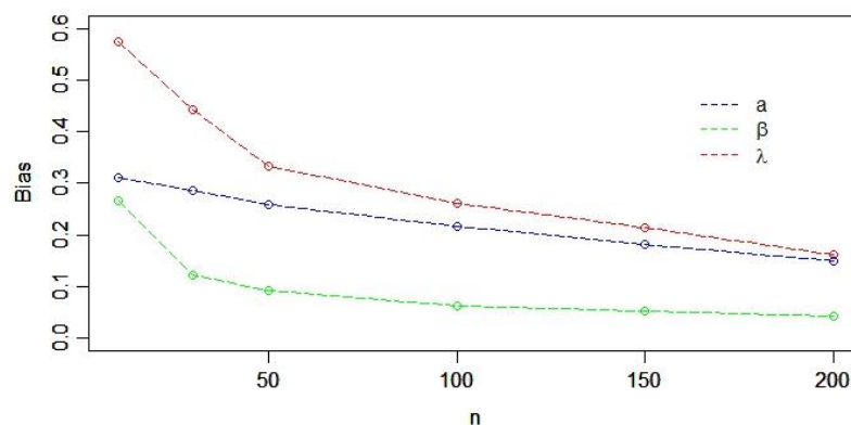
Figure 3. Absolute bias of selected parameters ( \alpha = 1, \beta = 2, \lambda = 2 ) for HCEE model.
