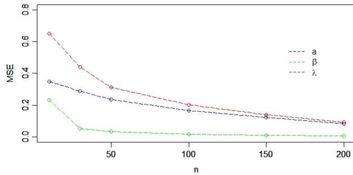
Figure 4. Absolute MSE's of selected parameters( a = 1, \beta = 2, \lambda = 2 ) for HCEE model.
