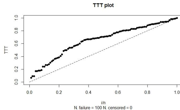
Figure 7. Scaled-TTT plot for the yarn data.
