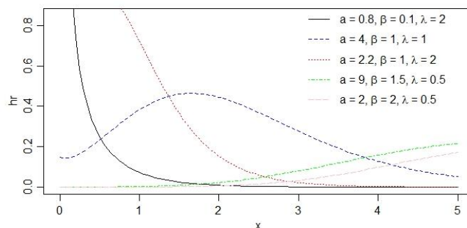
Figure 2. Failure rate function shapes for selected values of the parameters.
