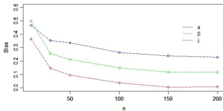
Figure 5. Absolute bias of selected parameters ( a = 2, \beta = 2, \lambda = 2 ) for HCEE model.
