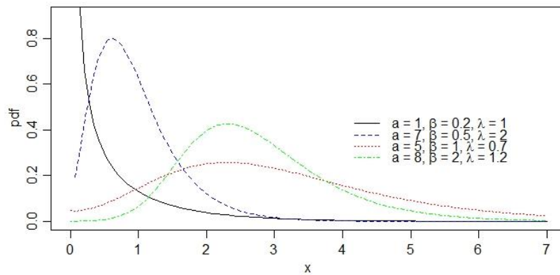
Figure 1. Plots of the HCW(a, \beta, \lambda) for different values of parameters.
