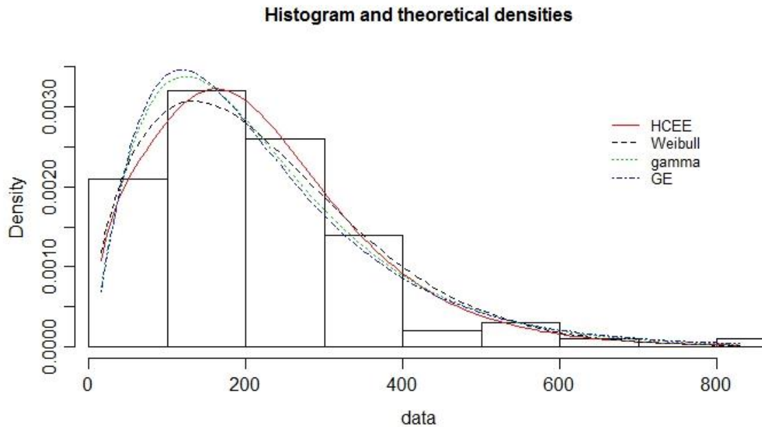
Figure 8(a). The fitted PDFs and the relative histogram for the yarn data set.
