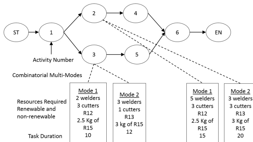
Figure 2. Task on Node of CMRCMPSP model
