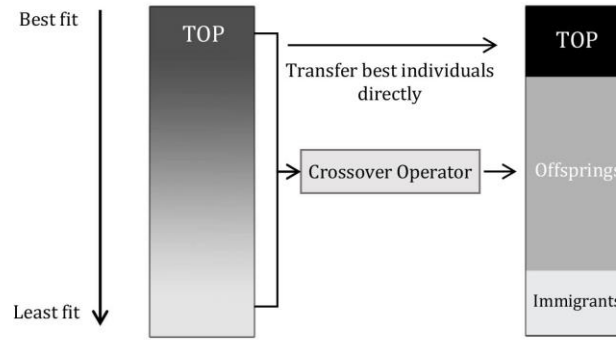
Figure 6. Transitional process between consecutive generations.
