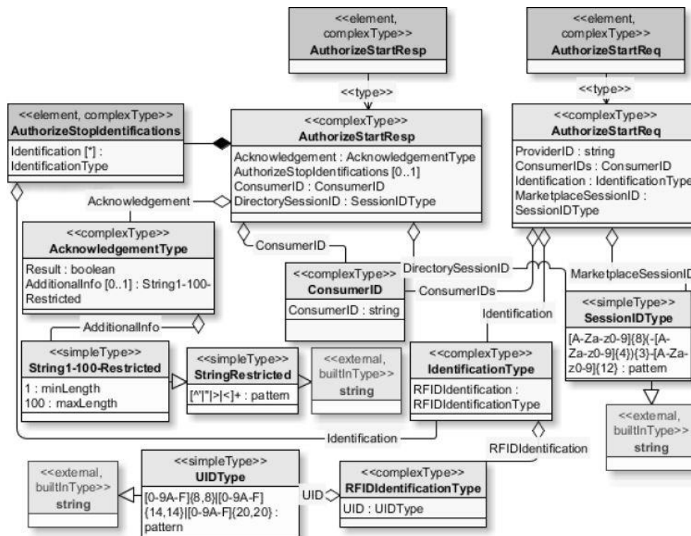
Figure 7. Object diagram for the authorization process.
