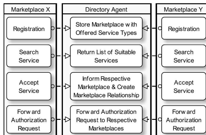
Figure 3. Interactions between marketplaces and directory agent.
