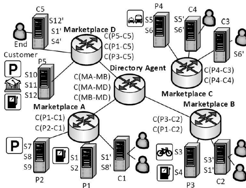
Figure 5. Architecture of the elaborated reference model.
