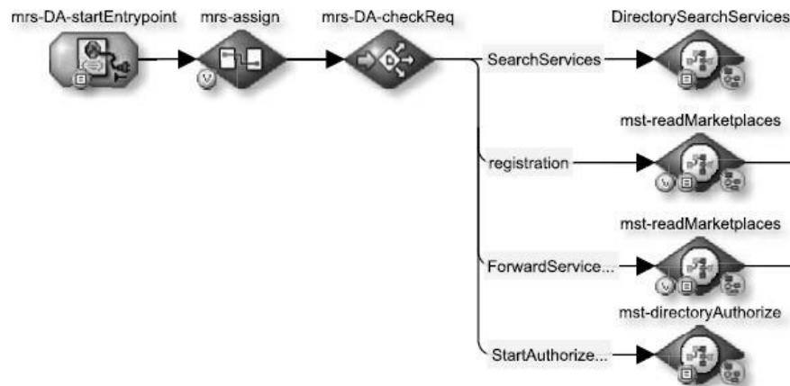
Figure 8. Directory agent technical workflow.
