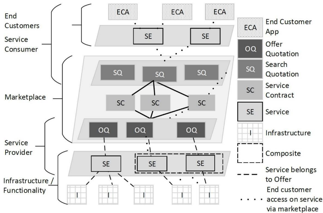
Figure 1. Abstraction of current logical connections and information flow.
