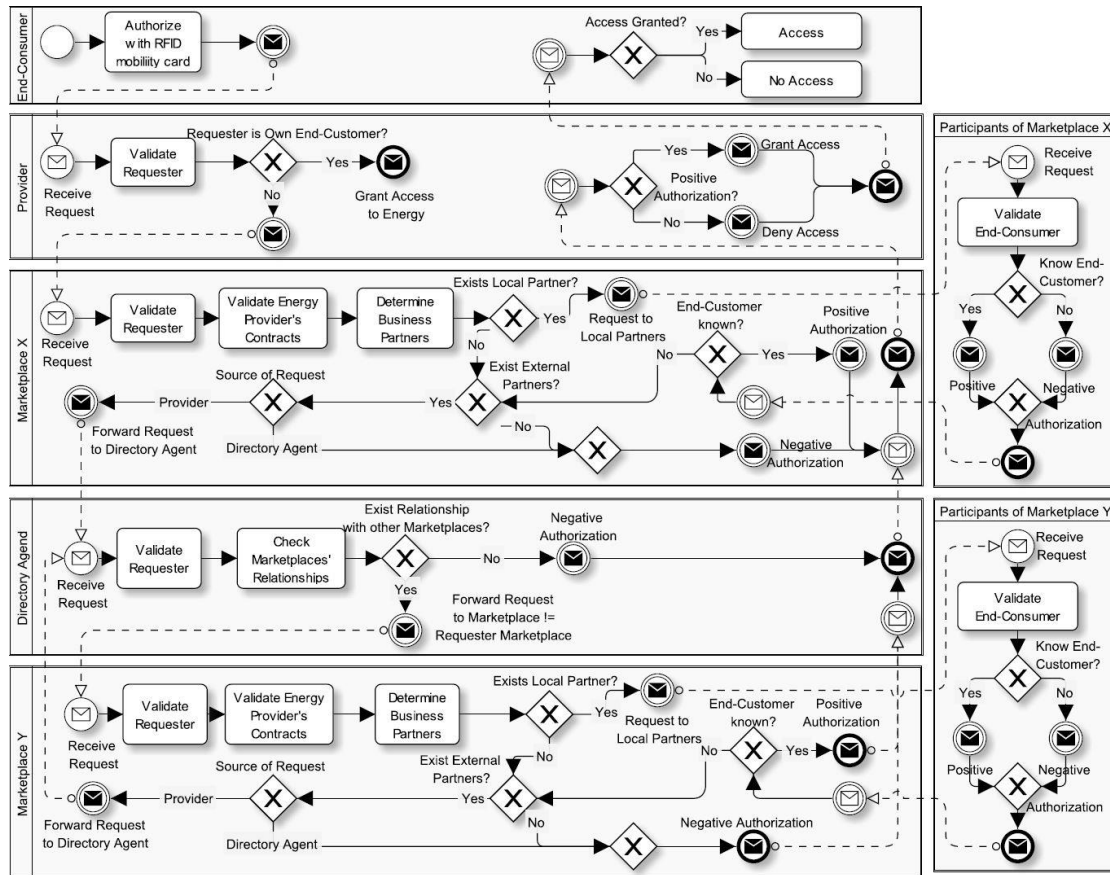
Figure 6. Authorization request roaming process throughout the complete ecosystem.
