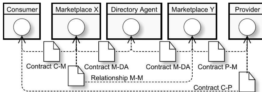
Figure 4. Artifacts depicting relationships.
