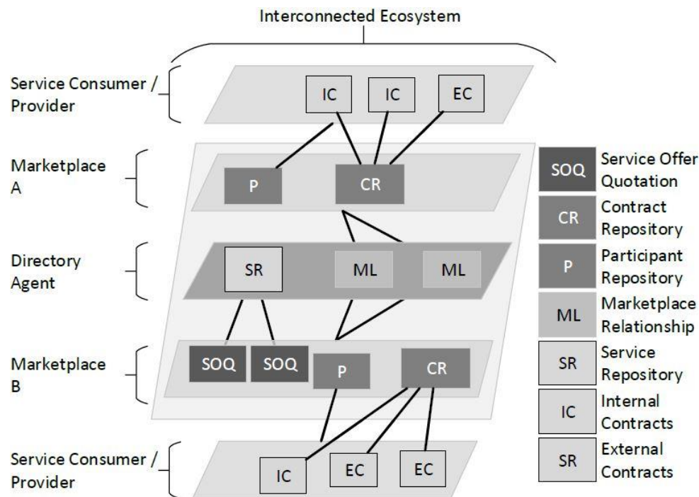
Figure 2. Abstraction of an interconnected service ecosystem.
