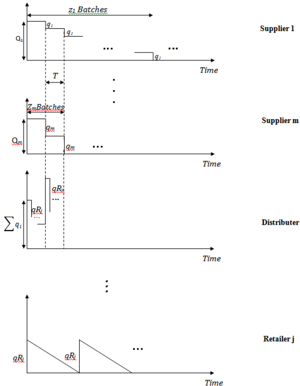
Figure 2. Inventory level in the supply chain players' storeroom: Traditional model
