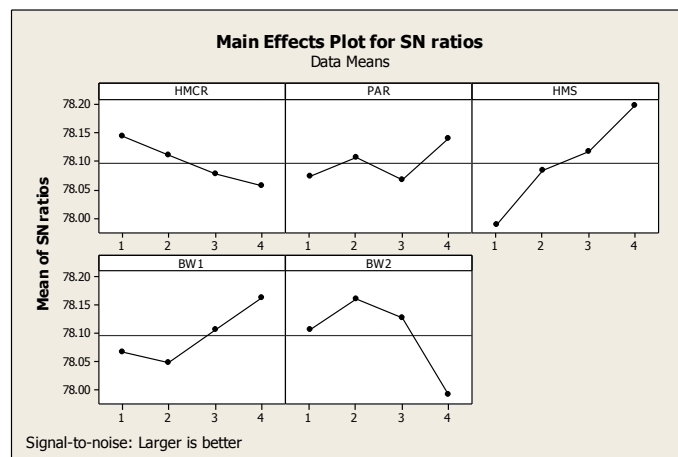
Figure 5. S/N of algorithm solution
