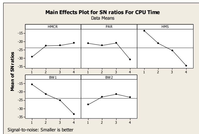
Figure 7. S/N of algorithm time
