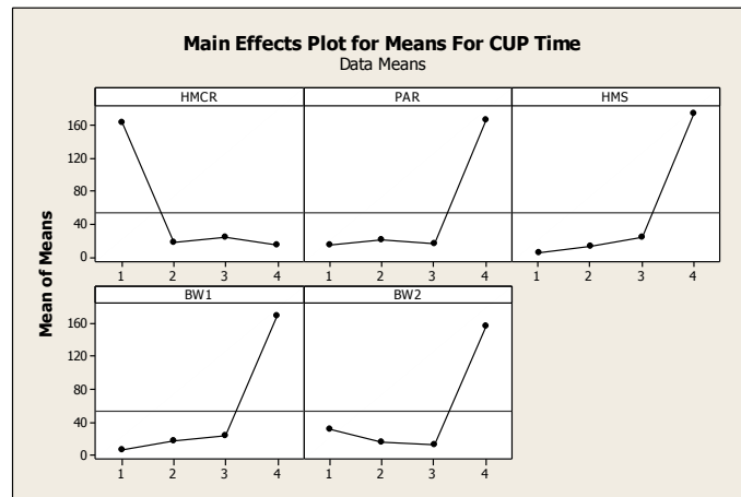
Figure 6. Mean of algorithm time
