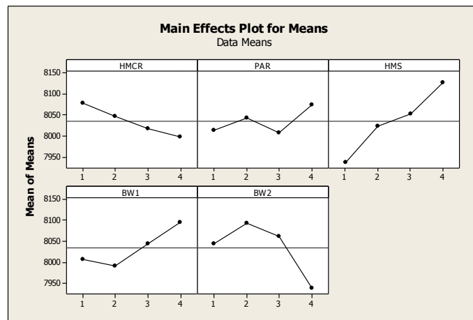
Figure 4. Mean of algorithm solution
